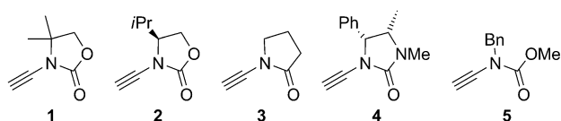
Figure 1. Ynamides considered in this work.
